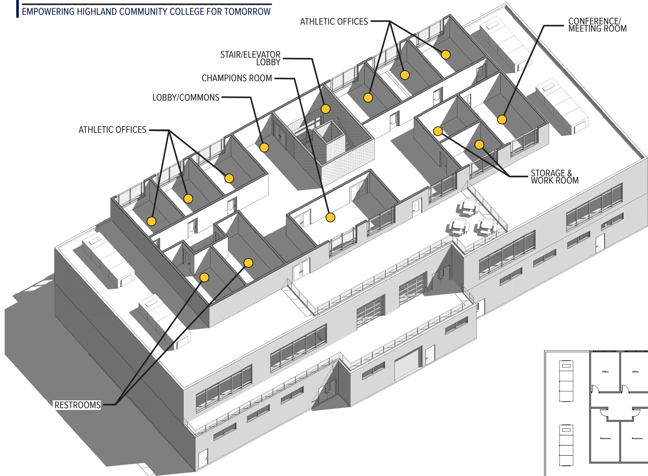
AXONOMETRIC VIEW: THIRD FLOOR
