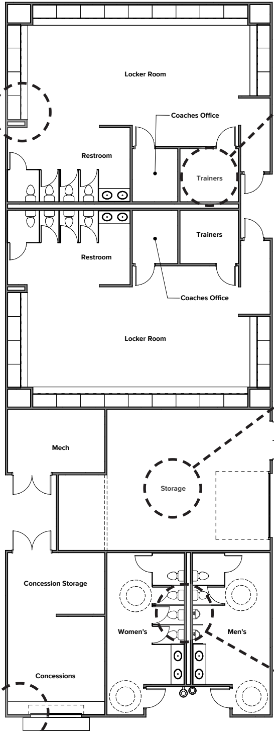
FLOOR PLAN: TRACK & SOCCER COMPLEX
